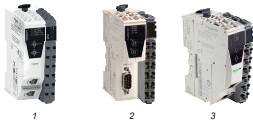
Communication interface module for distributed I/O on 1 Ethernet network 2 CANopen bus 3 Sercos III bus
