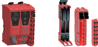
Safety logic controller Safety I/O module 1 Safety base 2 Safety electronic module 3 Safety terminal block
